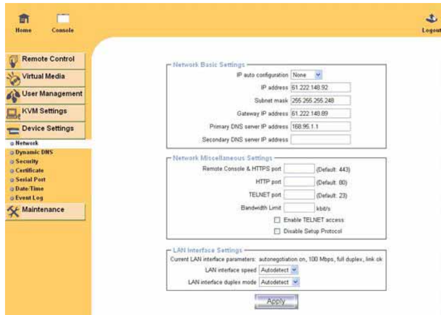
Figure 6-19. Network Settings
